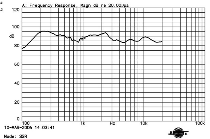
LF-K7070B43A 2.83Vrms by IEC268-5 1/2 std baffle 50cm X:1.0000kHz *Y:87.94dB ZA:Live Curve SSR Fund.
