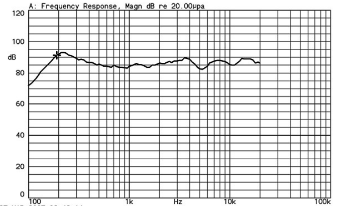
LF-K50B18C 2.83Vrms by IEC268-5 1/2 std baffle 50cm X:190.00Hz *Y:91.12dB ZA:Live Curve SSR Fund.
