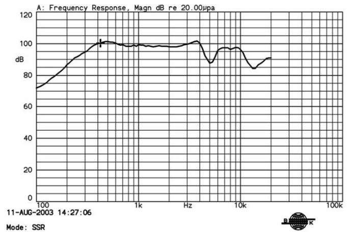
K40B10A 2.83Vrms by IEC268-5 1/2 std. baffle 10cm X:425.00Hz *Y:100.35dB ZA:Live Curve SSR Fund.
