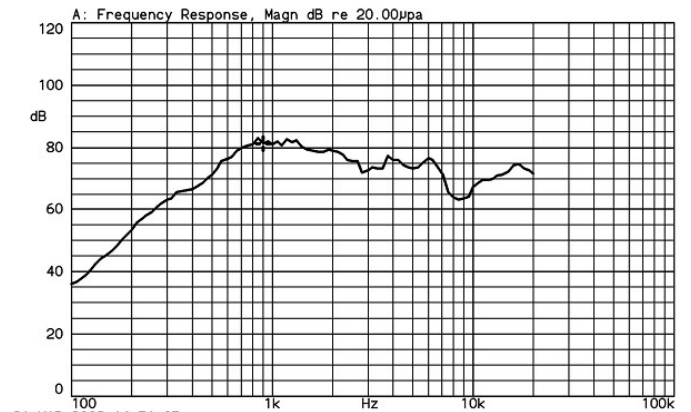
LF-K38B12A 1.26Vrms by IEC268-5 1/2 std baffle 50cm X:900.00Hz *Y:81.07dB ZA:Live Curve SSR Fund.
