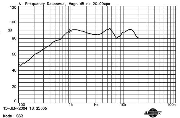
K15B34F 2Vrms by IEC268-5 1/2 std. baffle 10cm X:950.00Hz *Y:88.93dB ZA:Live Curve SSR Fund.
