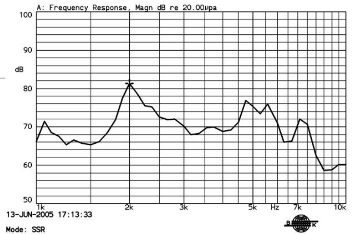
LF-MT12C01 1.5Vo-p square wave 10cm X:2.0000kHz *Y:81.33dB* ZA:Live Curve SSR T.Ha.
