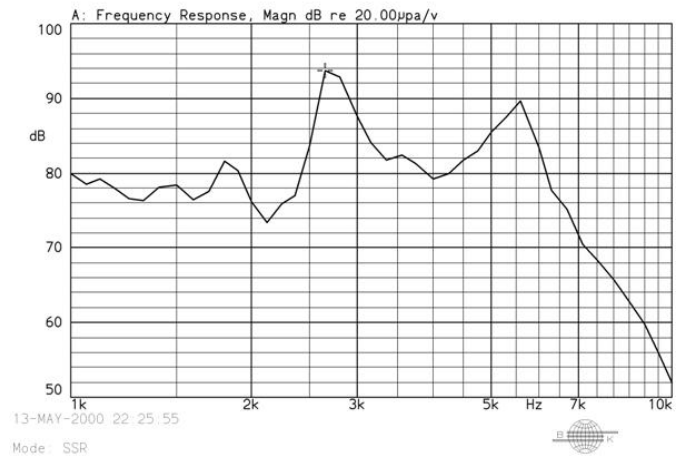
MT09D02 3.0Vo-p Square Wave 10cm test X:2.6500kHz *Y:93.78dB ZA:Live Curve SSR T.Ha.
