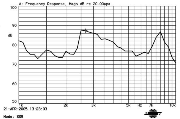
LF-MT09A03 5Vo-p square wave 10cm X:2.6500kHz *Y:87.39dB ZA:Live Curve SSR T.Ha.
