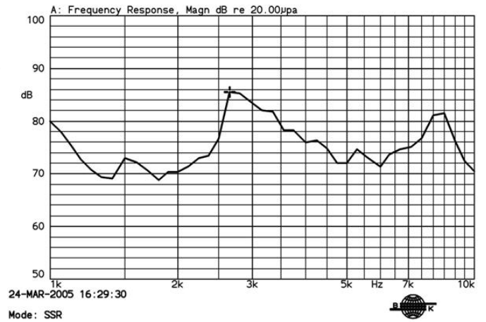
LF-MT09A02 3Vo-p square wave 10cm X:2.6500kHz *Y:85.56dB ZA:Live Curve SSR T.Ha.
