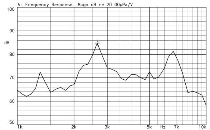
MT09A01 1.5Vo-p square wave 10cm test X:2.6500kHz *Y:84.85dB ZA:Live Curve SSR T.Ha.
