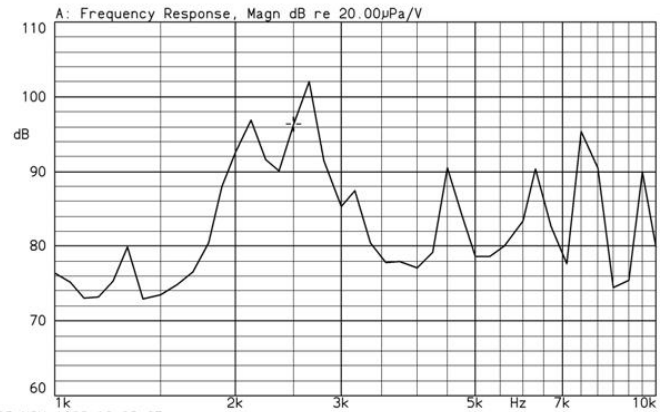
PE30P25A 9.0Vp-p Square Wave 10cm test X:2.500kHz *Y:96.34dB ZA:Live Curve SSR T.Ha.
