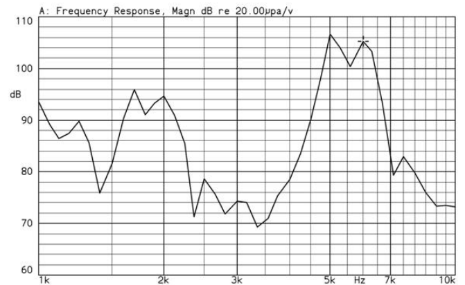
PE24P60A 9Vp-p Square wave 10cm test X:6.0000kHz Y:105.21dB ZA:Live Curve SSR T.Ha.
